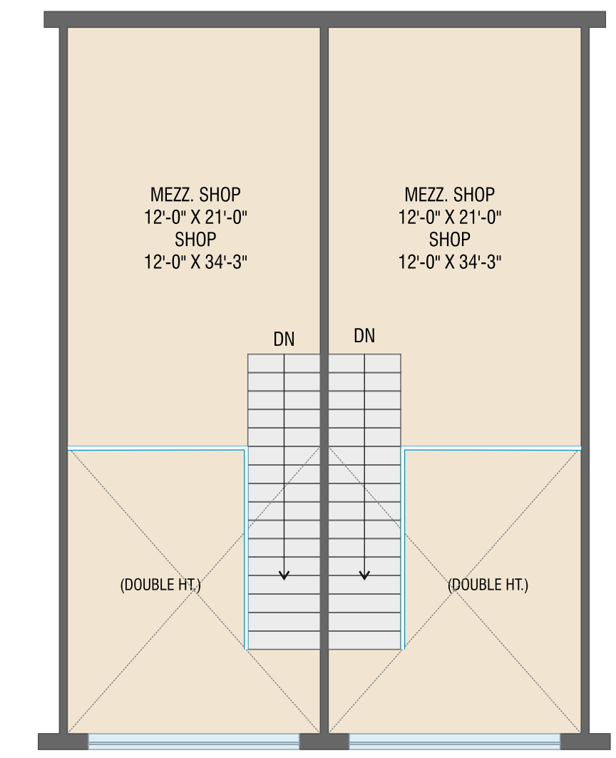
MEZZANINE FLOOR PLAN
